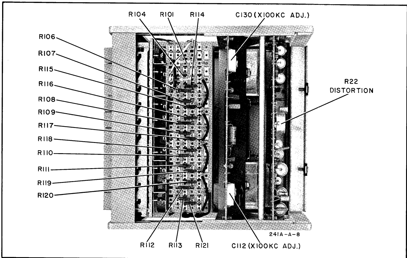
Figure 5-6. Top View
