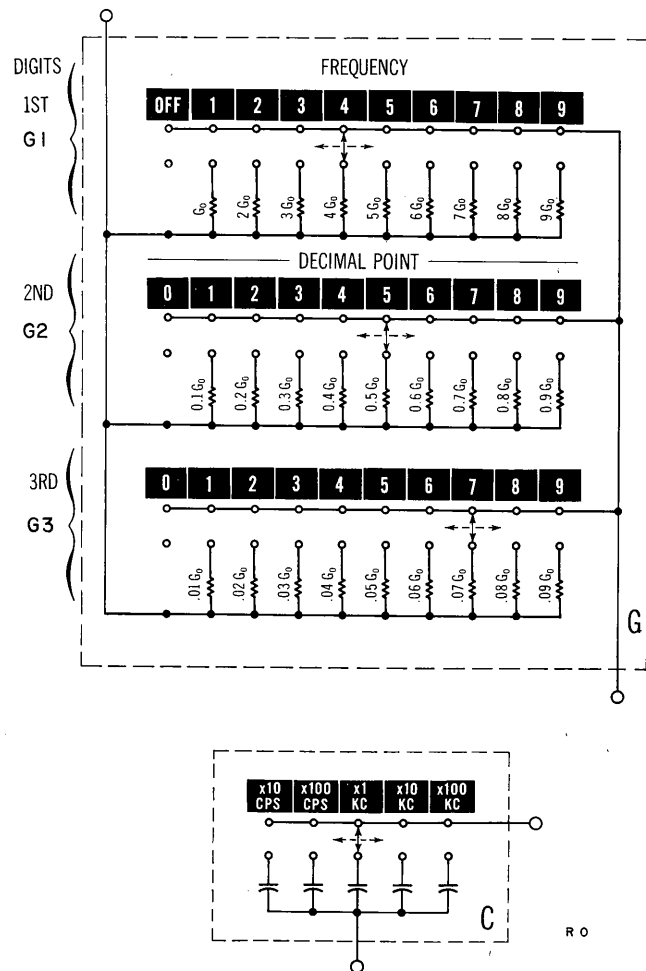
Figure 4-4. R and C Values of the Pushbutton Selector
