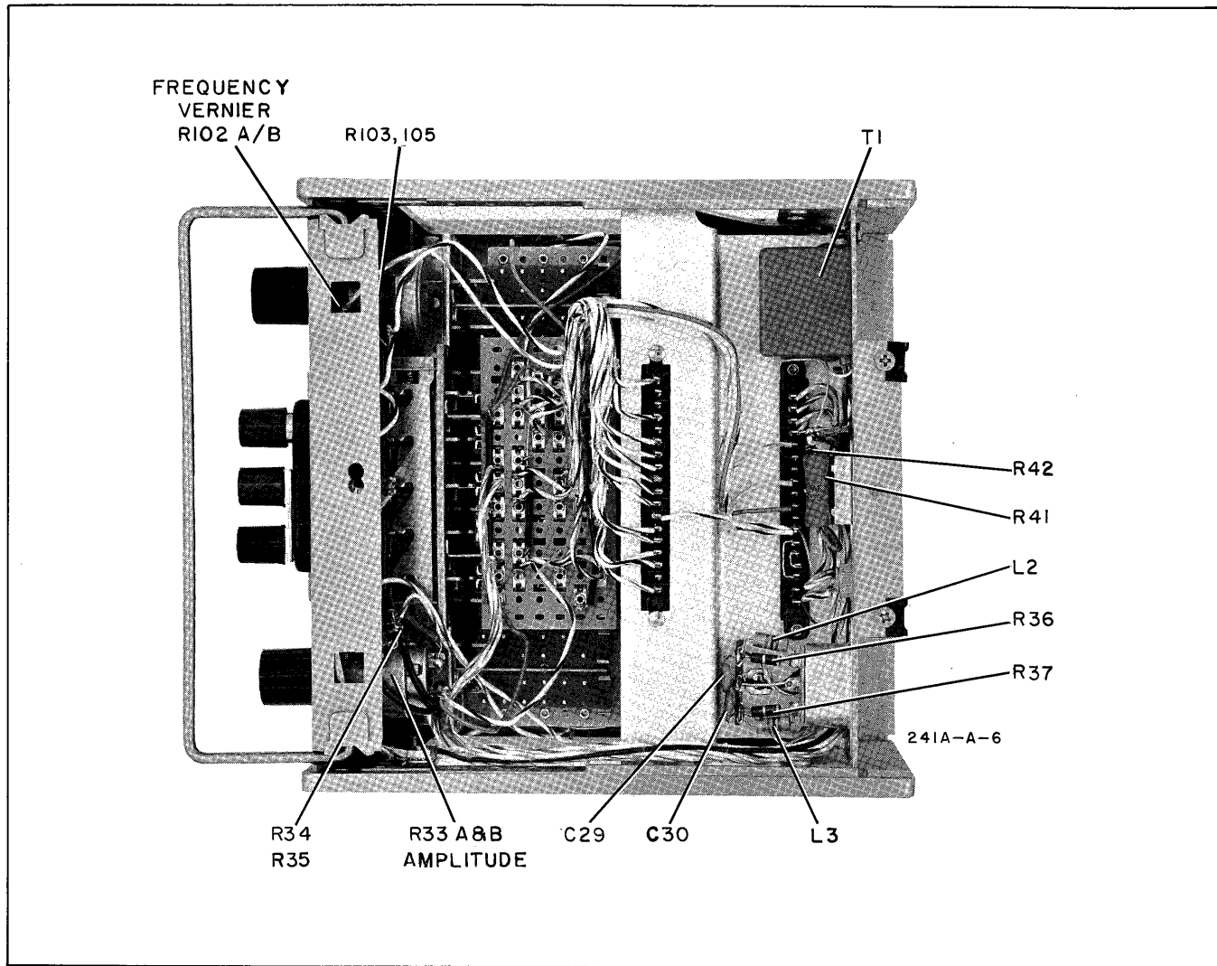
Figure 5-9. Bottom View
