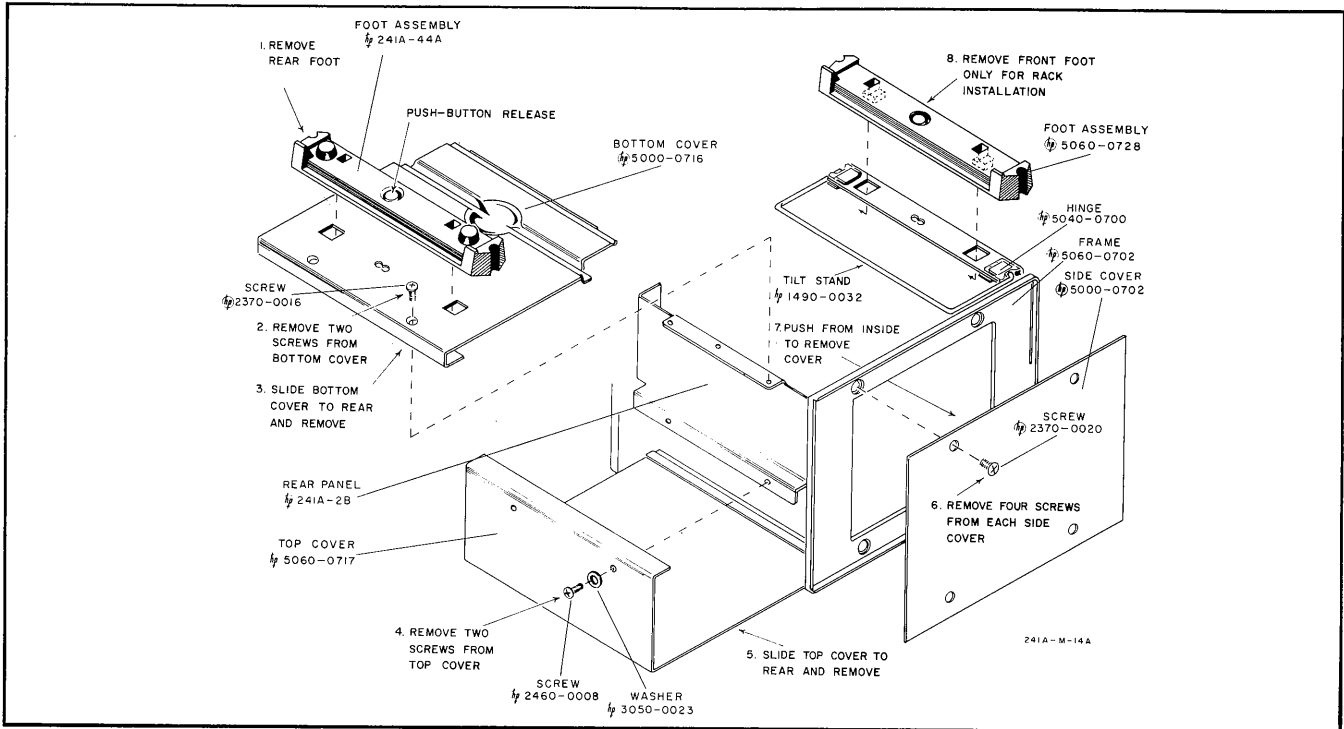
Figure 5-3. Cover Removal
