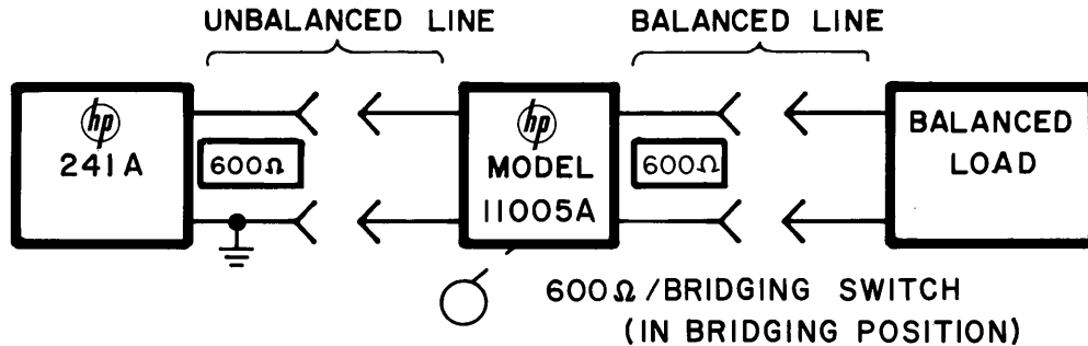
Figure 3-3. Balanced line configuration using 11005A
